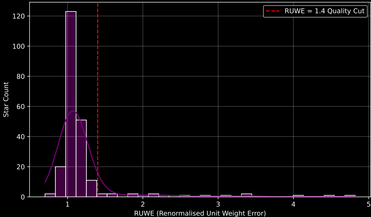
GAPOGEE DR17 Field [205-03-C] RUWE Distribution (n= 225)
