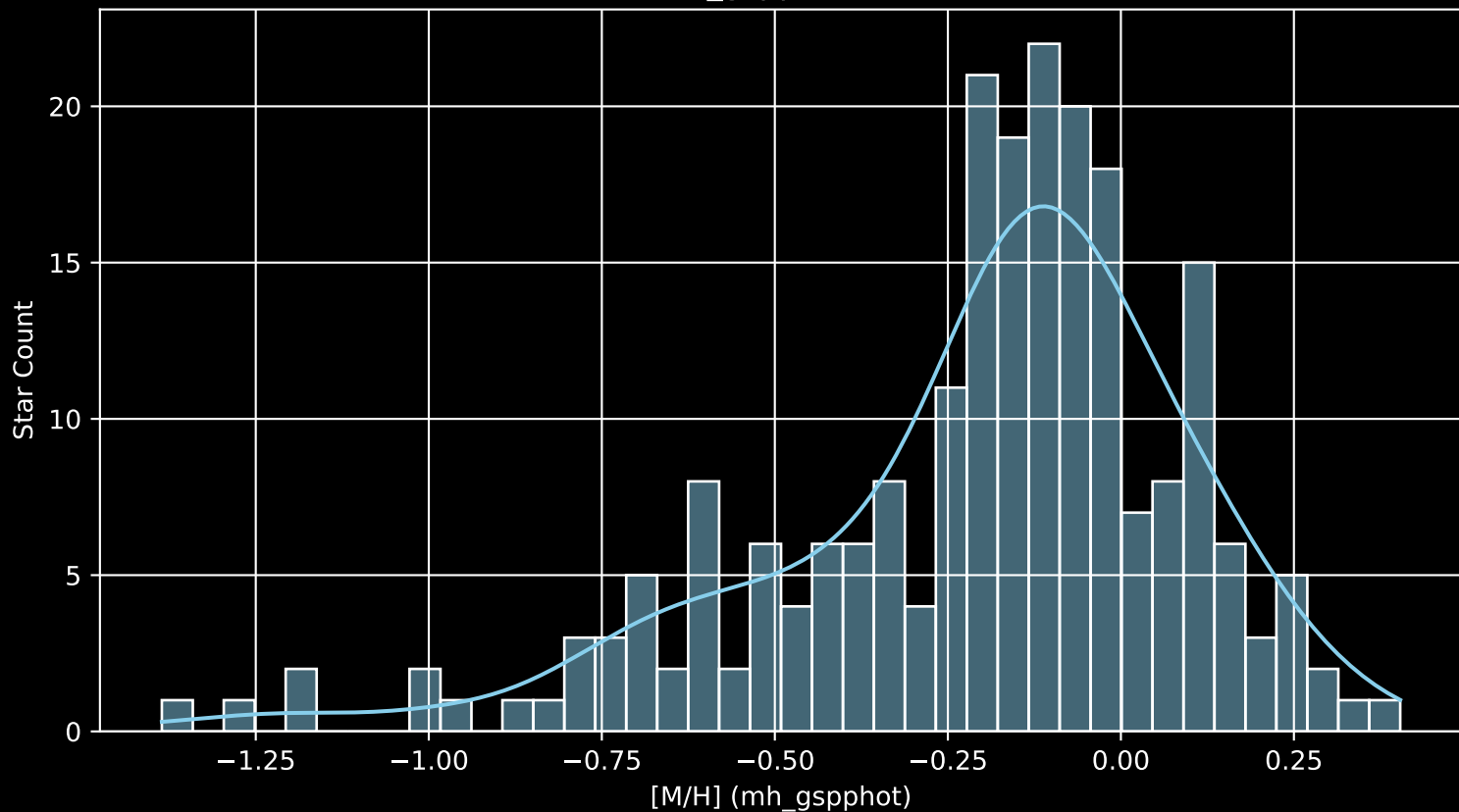
APOGEE DR17 Field: [205-03-C [M/H] (mh_gspphot) (n= 225)
