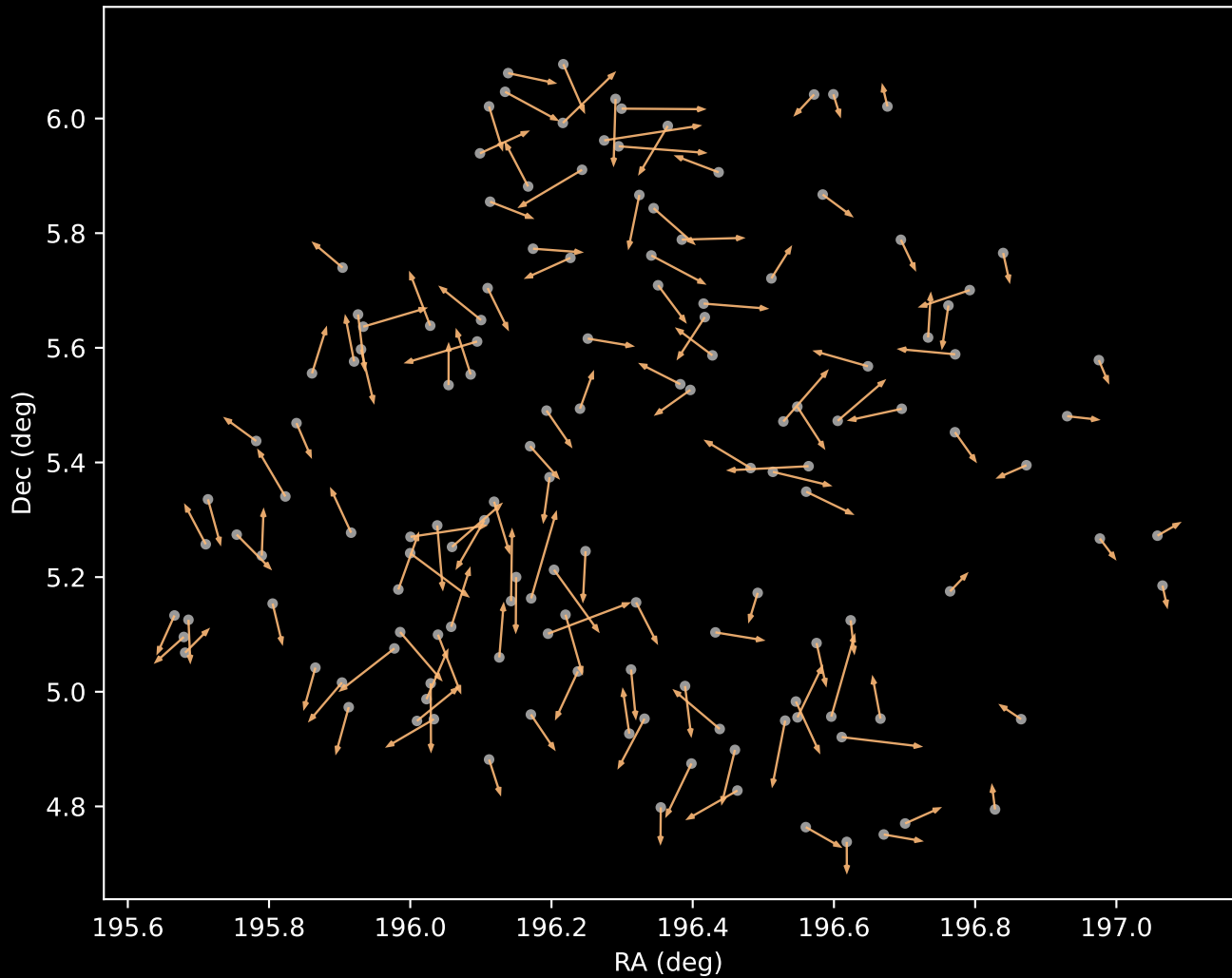
APOGEE DR17 Cluster 3 Proper Motion Vectors (n=140)
