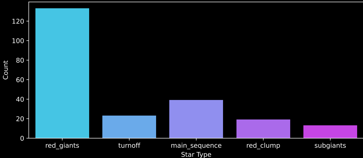
APOGEE DR17 Field: [205-03-C] Count plot of Star Type
