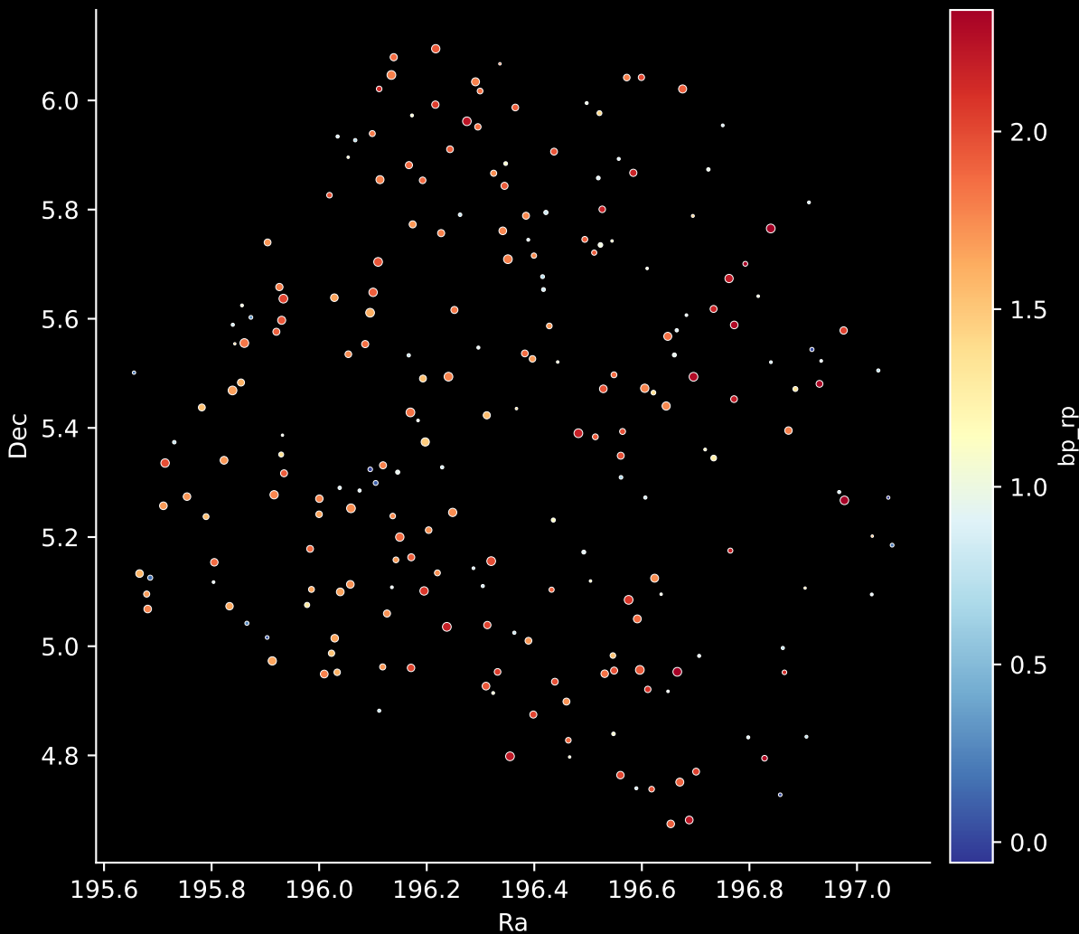
APOGEE DR17 Field: [205-03-C] Stars: 227
