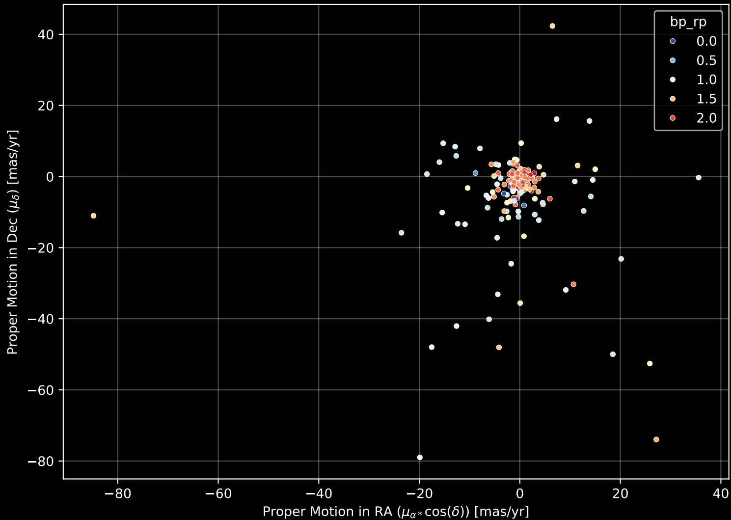
APOGEE DR17 Field: [205-03-C] Proper Motion Diagram (n= 227)
