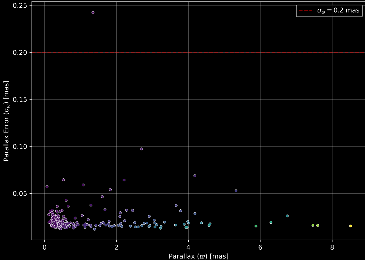
APOGEE DR17 Field: [205-03-C] Parallax Quality (n= 227)
